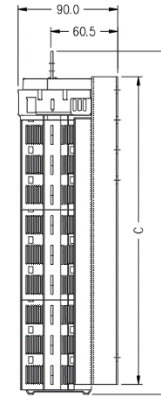
CHASSIS SIDE VIEW
