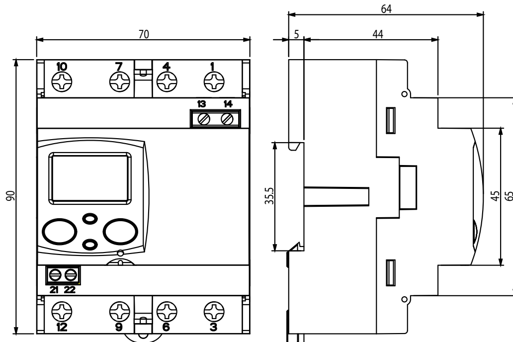
Figure 18: Dimensions of the CEM-C21.
