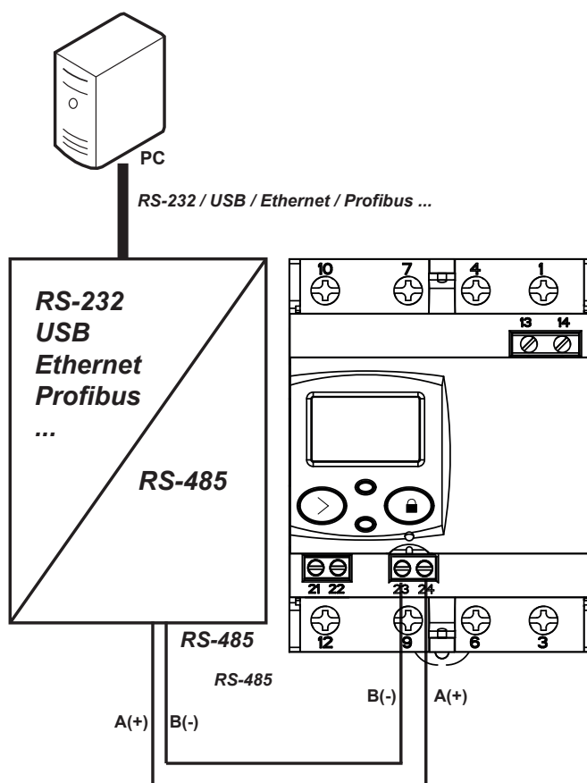
Figure 17: CEM-C21-485-T1 and CEM-C21-485-DS connection diagram.
